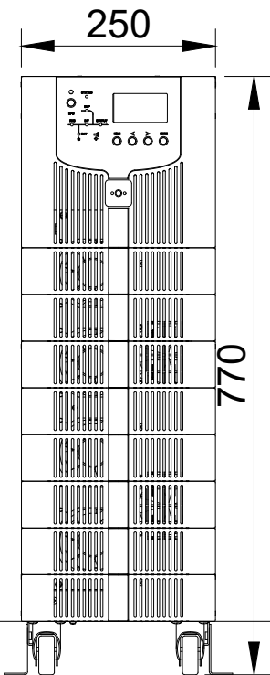
FRONT
